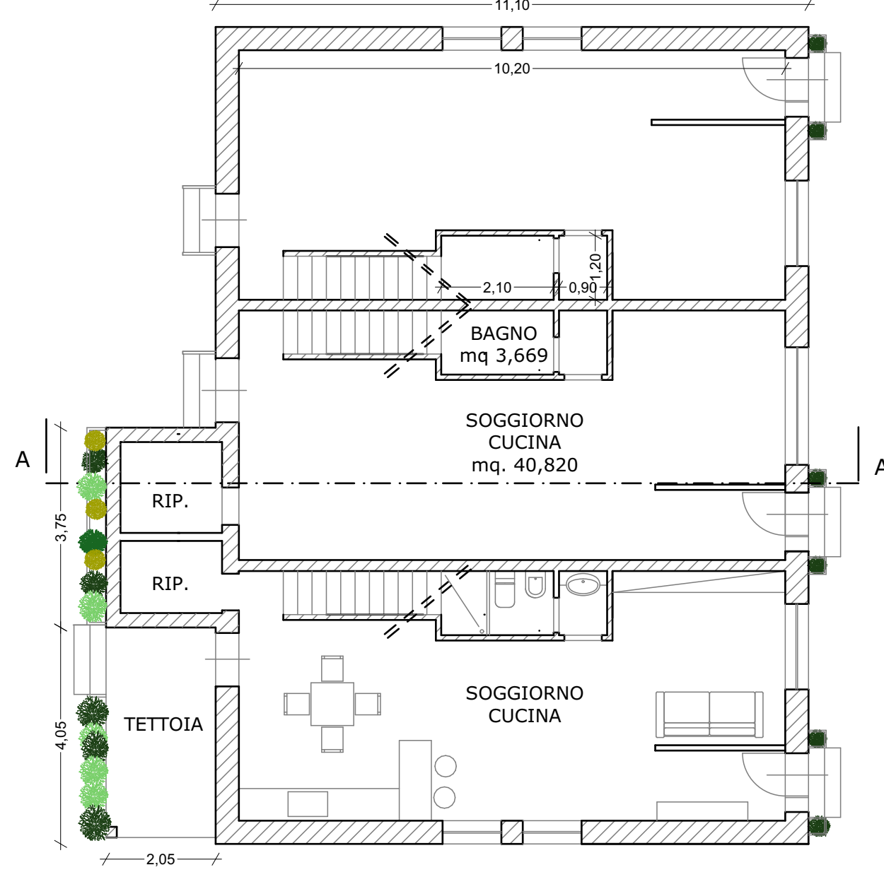
PIANO TERRA
